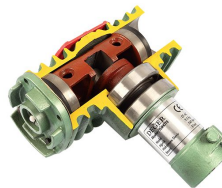
Product Tractor Power Take-Off Compressor
