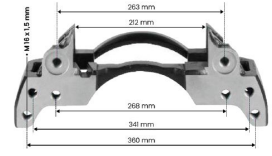
Product Caliper Carrier
