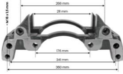
Product Caliper Carrier
