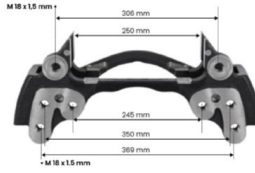
Product Caliper Carrier
