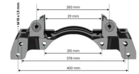
Product Caliper Carrier
